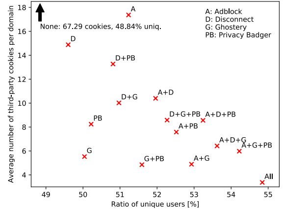
Figure 12: Uniqueness of users vs. number of unblocked third-party cookies
