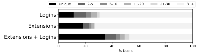
Figure 5: Distribution of anonymity set sizes for 16,393 users based on detected extensions and logins.
