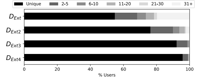
Figure 8: Anonymity sets for users with respect to the number of detected extensions
