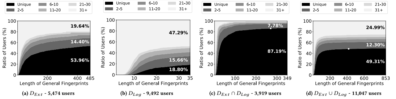
Figure 11: Anonymity sets for different numbers of attributes tested by general fingerprinting algorithm.
