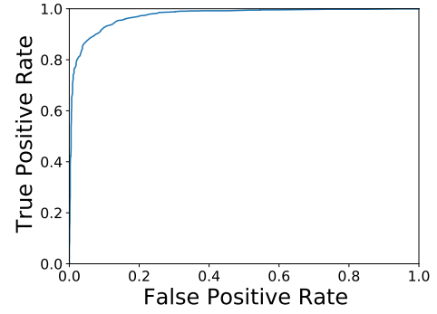
Fig. 2. The ROC curve for the sex prediction model (AUC=97.6%)
